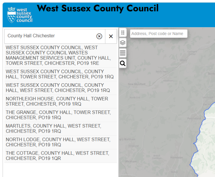
Figure 4: Search results
