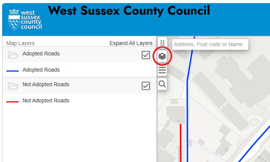
Figure 6: Map Layers
