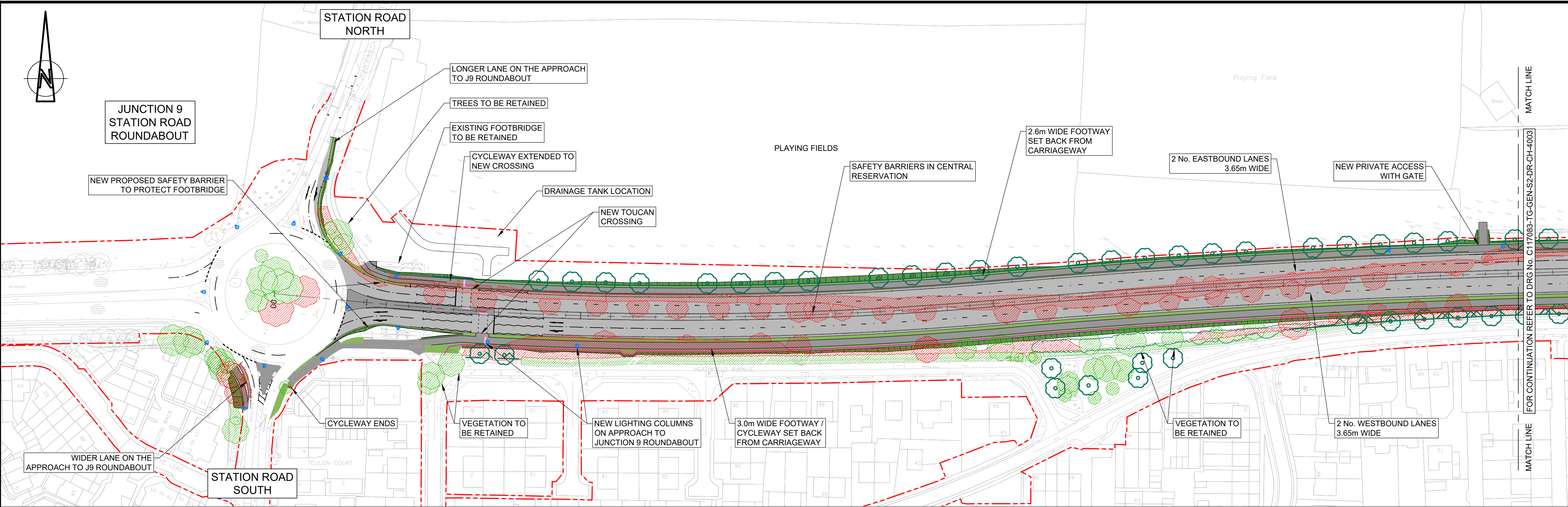
PHASE 1 DUALLING JUNCTION 9 (STATION ROAD ROUNDABOUT) TO JUNCTION 10 (ROUNDSTONE LANE ROUNDABOUT) SCALE 1:1000
